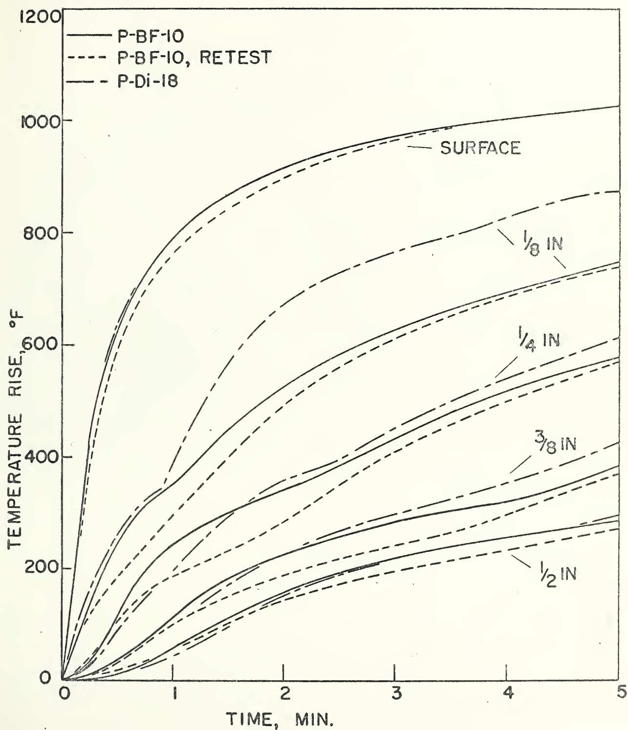
FIG 1. TEMPERATURE - TIME DATA
