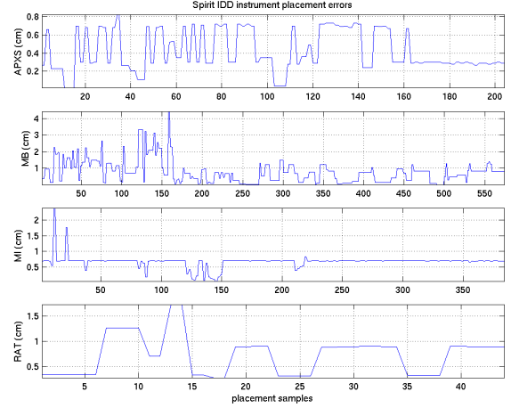
Fig. 12. Robotic arm positioning errors for Spirit when placing the APXS, MB, MI, and RAT instruments onto science targets. Data covers instrument placements through sol 944.
