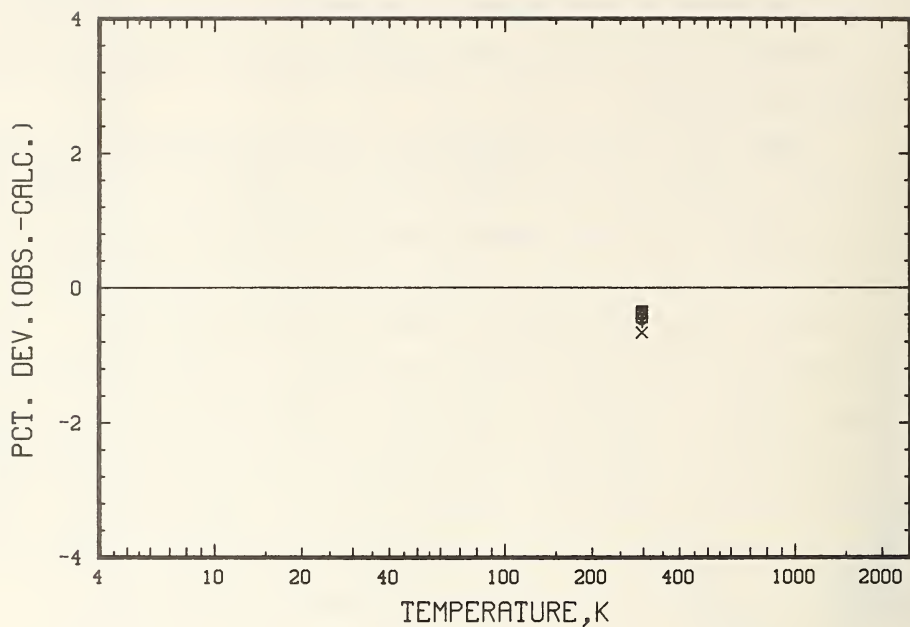
Figure 48. Electrical resistivity deviations for seven AXM-5Q1 graphite specimens as reported by Hust (7) from eq. (5.2.2) at 296 K.
