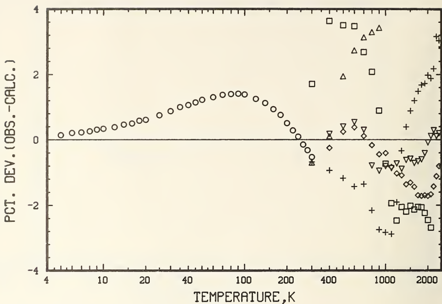
Figure 50. Electrical resistivity deviations for six AXM-5Q1 graphite specimens as reported by the following participants from eq. (5.2.2) at temperatures from 5 to 2500 K.
