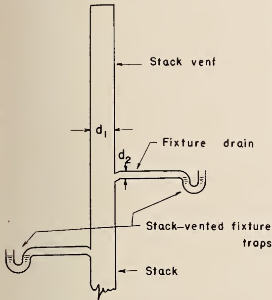
FIGURE 2. Stack-vented fixture traps.
