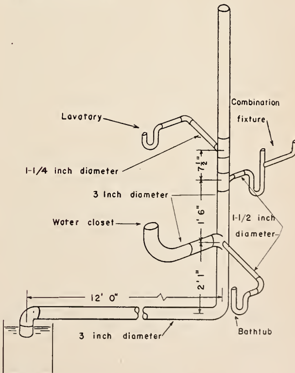
FIGURE 10. Test setup for simulating submerged house sewer.
