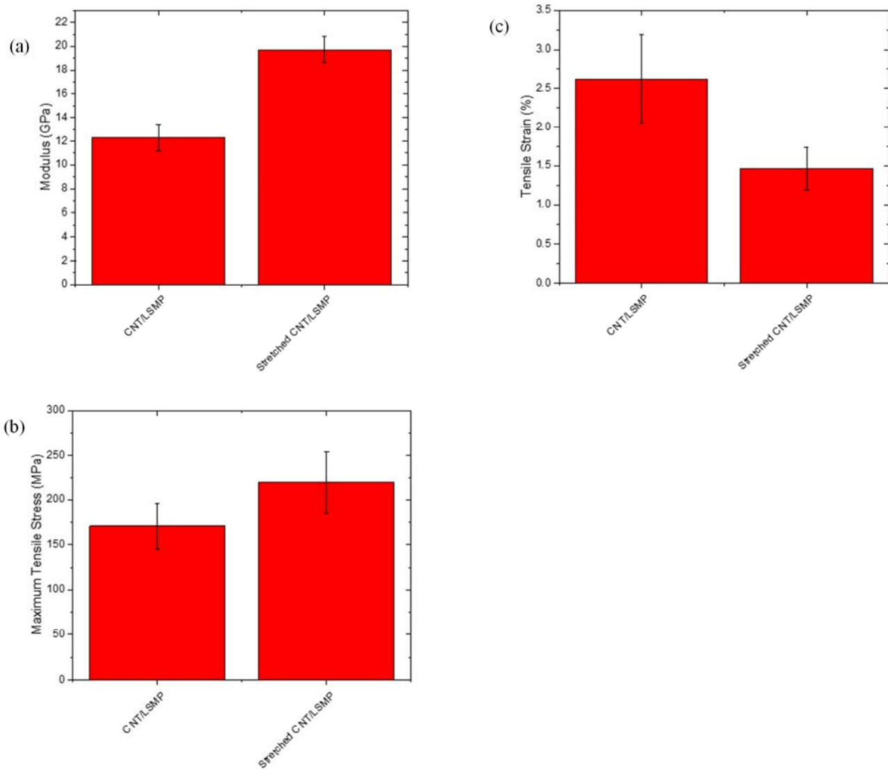
Figure S6. Tensile properties of CNT sheet/LaRC-SMP and stretched CNT sheet (40%)/LaRC-SMP. (a) modulus, (b) maximum tensile stress and (c) strain at break.
