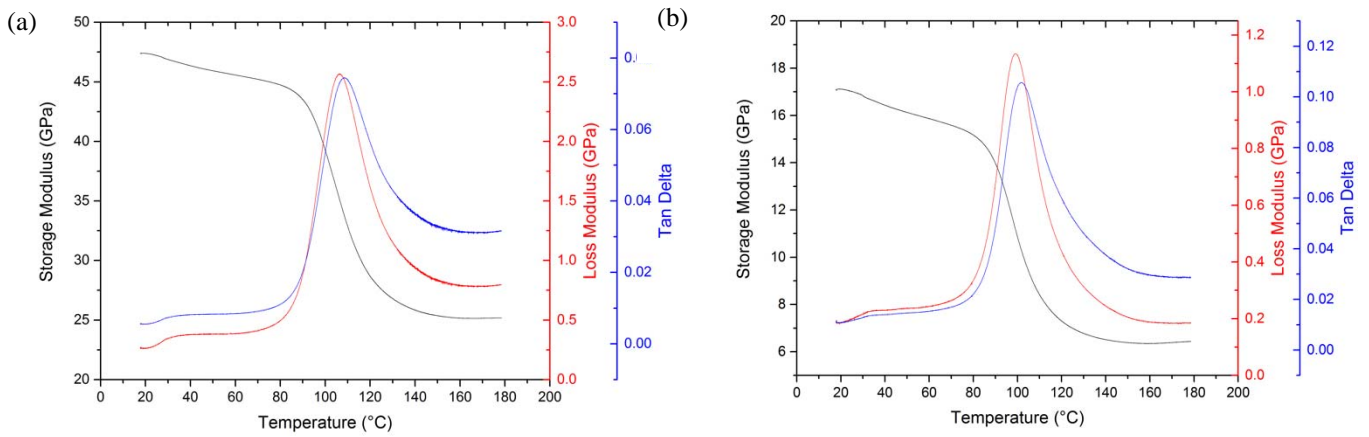
Figure 18. Dynamic mechanical analysis of carbon fiber ([+45°/0°/-45°/90°] 2s ) reinforced SMP composite of (a) 0° cut and (b) 90° cut.
