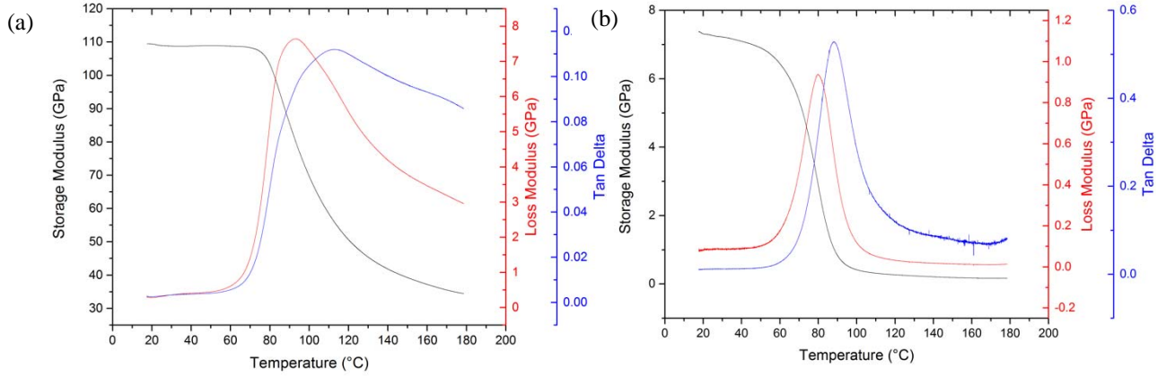
Figure 17. Dynamic mechanical analysis of carbon fiber (UD, [0°] 8 ) reinforced SMP composite of (a) 0° cut and (b) 90° cut.
