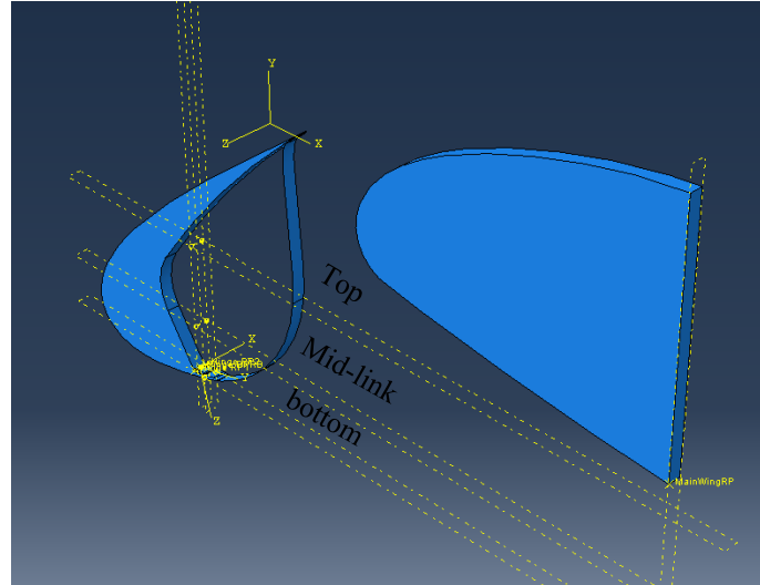
Figure 22. Abaqus model of SCF for retraction/deployment performance.
