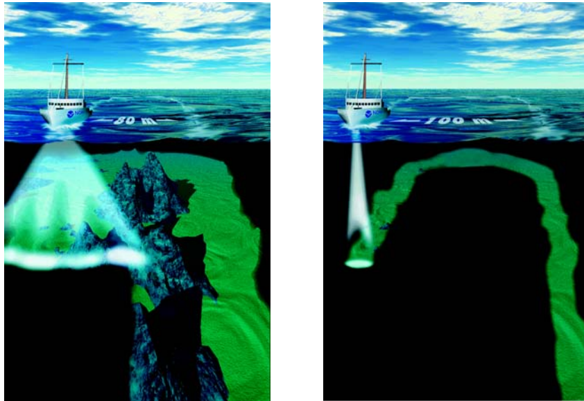
Figure 8. Multi-beam echosounder (left) and single-beam echosounder (right). The signal swath of the multi-beam sonar is broader than that of the single-beam; thus, the multi-beam signal provides greater seafloor coverage.
