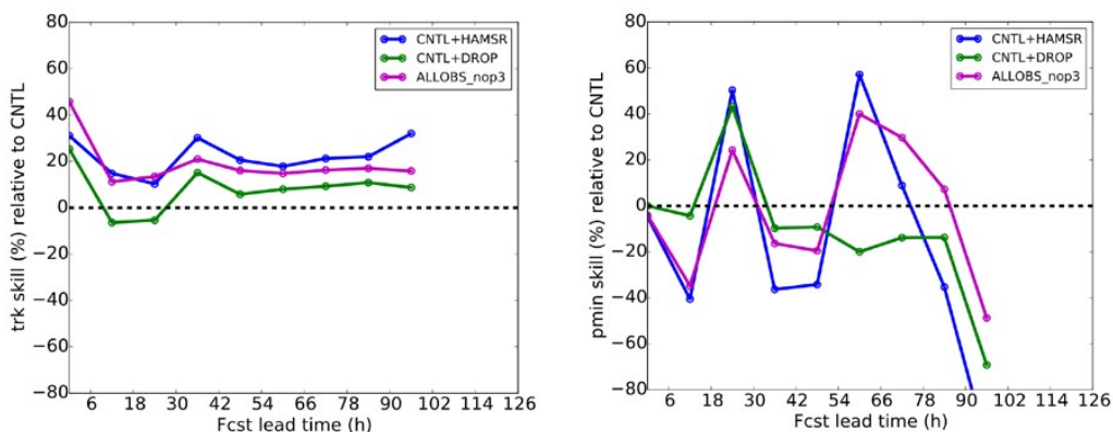
Figure 2.13. Results summarizing the impact of HAMSR retrievals within HWRF-HEDAS. The results are averages over 5 model cycles from the 2016 Hermine flights. The panels show the relative impact on the forecast track (left) and minimum pressure (right) skill for addition of the HAMSR (blue) and the dropsonde observations (DROP, green) to the control (CNTL) forecast. The magenta trace reflects addition of both HAMSR and dropsondes. Graphics provided by Hui Christophersen and Altug Aksoy.
