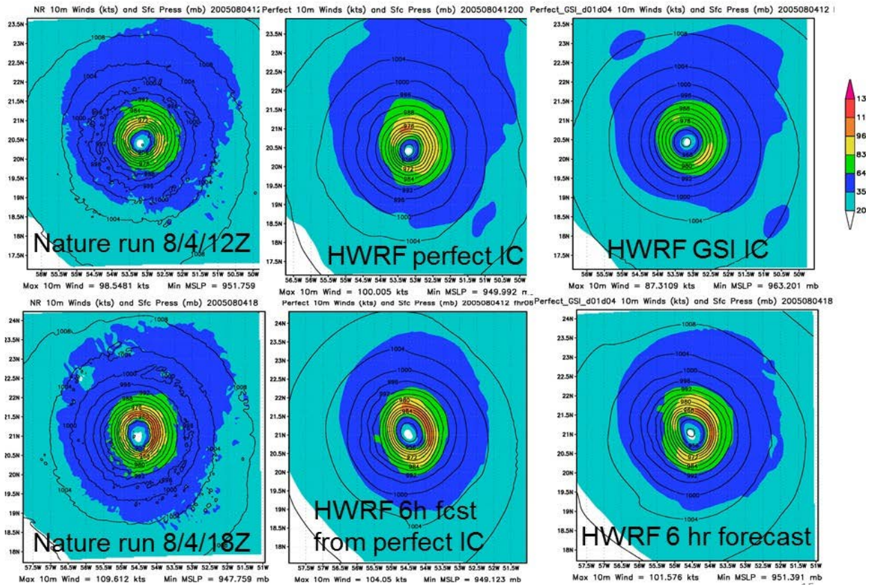
Figure 3.2. Evolution of the simulated hurricane wind speeds over a 6-hour period for the WRF nature run (left), HWRF with near perfect initial conditions (IC; middle), and HWRF with initial conditions from the GSI system (right). Graphics provided courtesy Robert Atlas.
