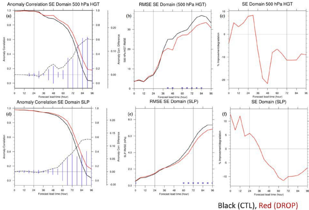
Figure 2.21. Impact of assimilation of Global Hawk dropsondes (DROP) versus the control (CTL) model on anomaly correlation scores and root mean squared error (RMSE) from GFS forecasts during Hurricane Matthew relative to the full observing system. The left panels show the anomaly correlation, the center panels display the RMSE, and the right panel shows the percent change in the RMSE as a function of forecast lead time. Upper panels are for the 500 hPa height field (HGT) and lower panels are for the sea level pressure (SLP). The results reflect averages from three model cycles and over the southeast (SE) verification region. In the anomaly correlation plots, differences (dashed lines) outside of blue vertical lines are significant at the 95% confidence level. Blue stars in the RMSE plots indicate lead times that are statistically significant at the 95% level. Graphics provided by the GOSA Group as appearing in Kren et al. 2017.
