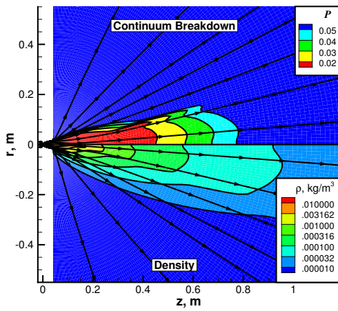
a) Expanding perfect gas jet ( N_2 ).
