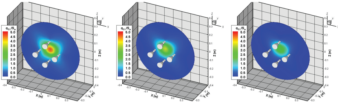
a) Thruster base T_{\text{wall}} = 100 K.
