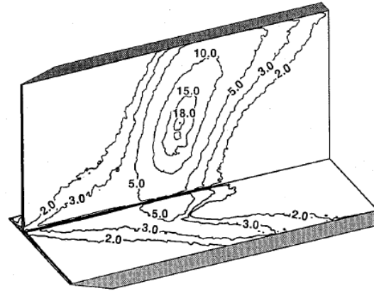
b) DSMC surface pressure [10]
