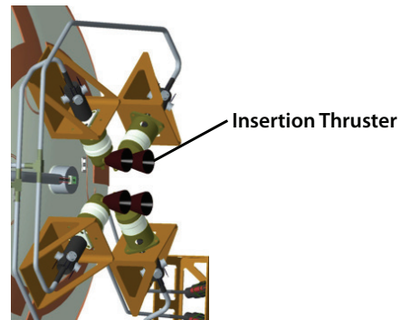
b) Close-up view of four tightly-clustered insertion thrusters.
