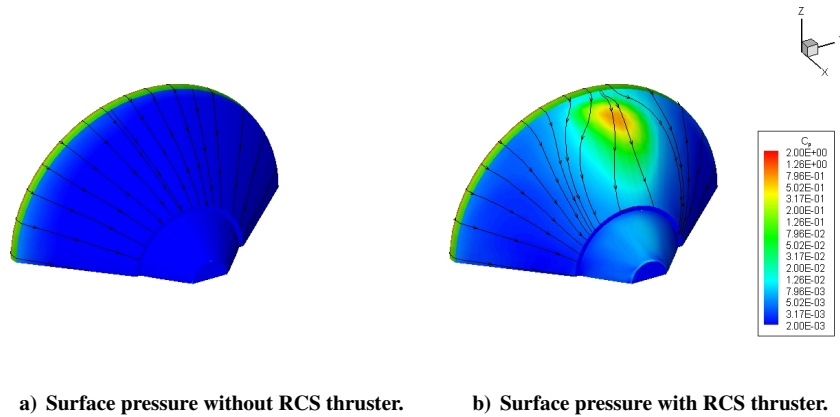
Figure 24. DSMC of Phoenix afterbody at Kn_L = 0.1 .
