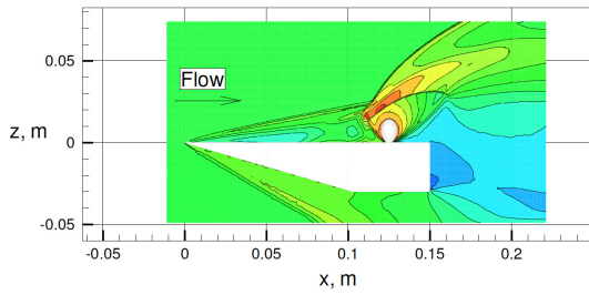
a) Flow-field symmetry plane number density contours.
