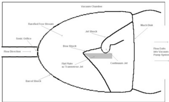
a) Sketch of RCS model.
