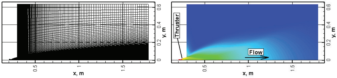
a) Axisymmetric grid for insertion thruster.
