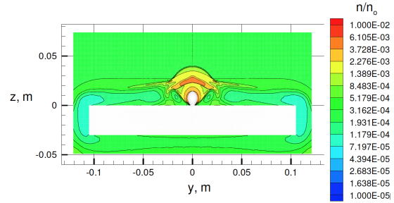
b) Flow-field cross-flow plane number density contours at nozzle.
