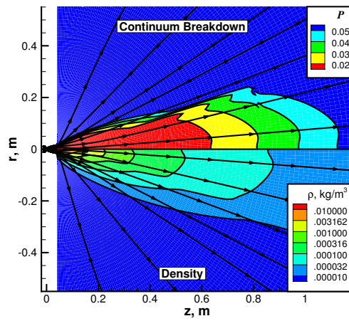
b) Expanding hydrazine reaction gas jet ( NH_3-N_2-H_2 mixture).
