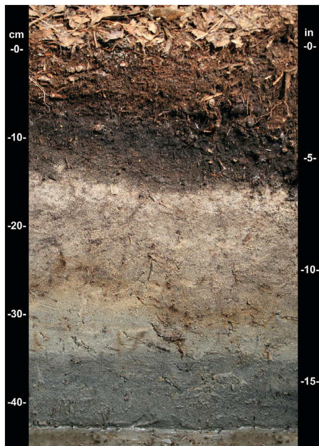
Figure 2.— The soil profile above consists of an 8 cm (3.14 inches) layer of peat and/or mucky peat underlain by a 1 cm (0.4 inches) layer of muck. The remaining soil layers are sandy soil material. In LRRs R, W, X, and Y, observations would begin below the peat, mucky peat, and muck layers (9 cm). In LRRs F, G, H, and M, observations would start at the actual soil surface. In all remaining LRRs, observations would begin at the muck surface (8 cm).
