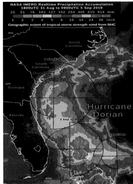
Fig. 2 Rainfall footprint of Hurricane Dorian (2019) as measured by NASA satellite-based instrumentation associated with the Global Precipitation Measurement Mission (GPM).
