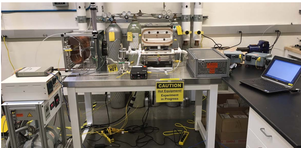
Figure 45. Laboratory test layout for testing the integrated hydrogen sensor and separation module.
