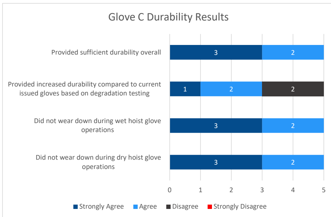
Figure 3-14 Glove C Durability Results
