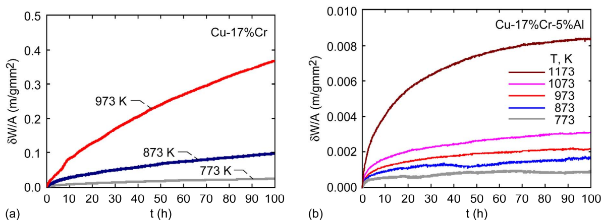
Figure 2.—Specific weight change versus time plots at temperatures ( T ) between 773 and 1173 K. (a) Cu-17%Cr. (b) Cu-17%Cr-5%Al.
