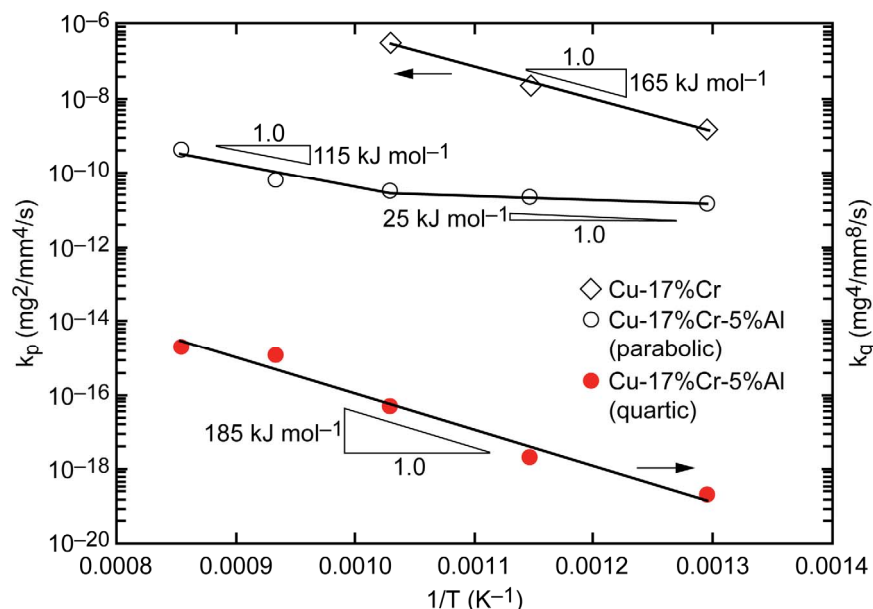
Figure 7.—Arrhenius plot showing the temperature dependence of the parabolic and quartic rate constants for Cu-17%Cr and Cu-17%Cr-5%Al.
