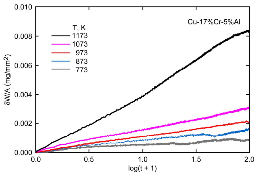
Figure 10.—Plot of the specific weight change versus \log(t + 1) at different temperatures ( T ) demonstrating the applicability of the direct logarithmic relationship to describe the oxidation behavior of Cu-17%Cr-5%Al.
