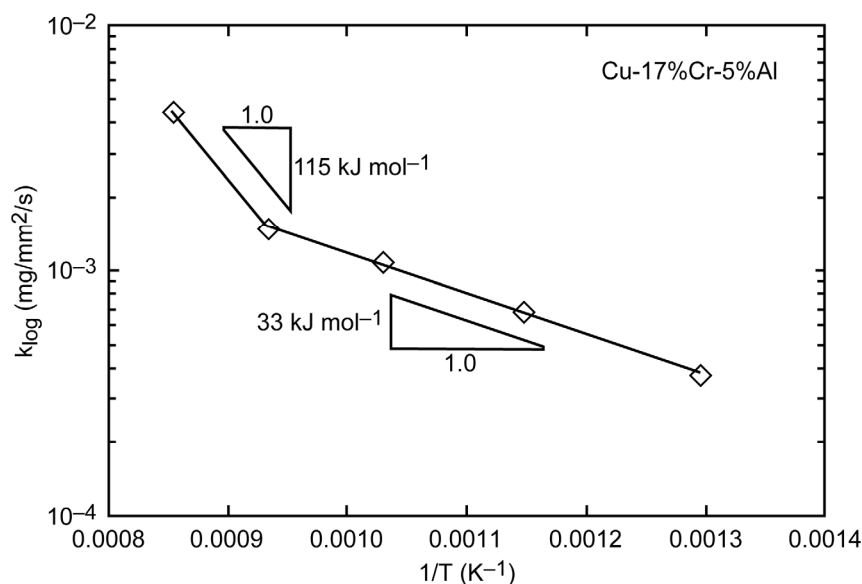
Figure 12.—Arrhenius plot of the logarithmic rate constant versus the inverse of the absolute temperature for Cu-17%Cr-5%Al.
