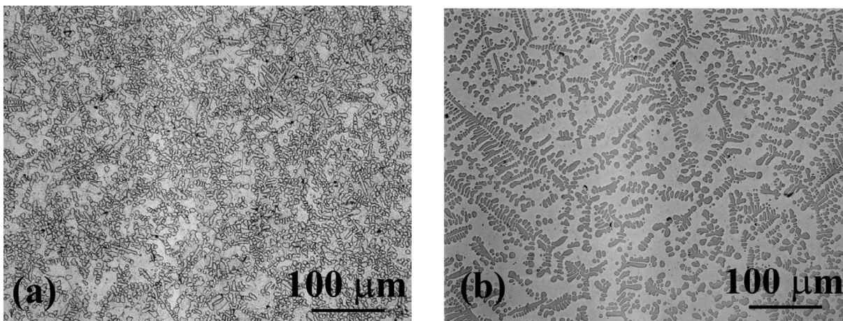
Figure 1.— Optical microstructures of as-cast alloys. (a) Cu-17%Cr. (b) Cu-17%Cr-5%Al.
