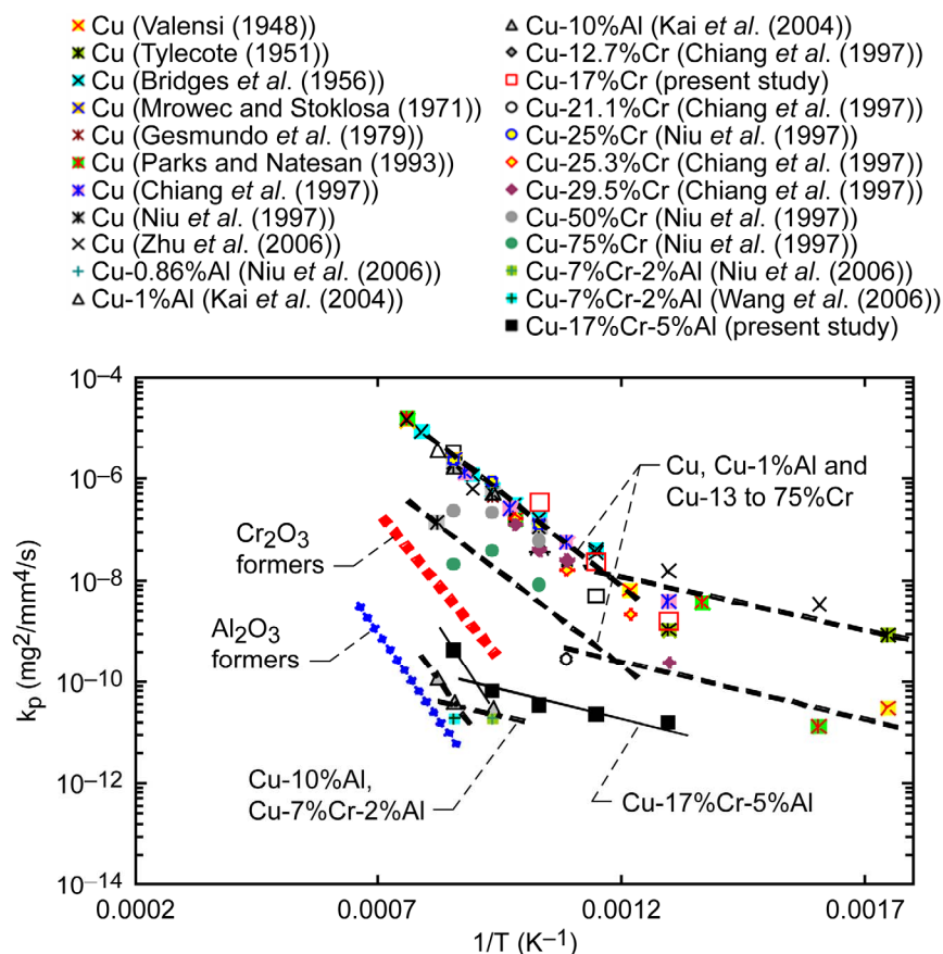
Figure 8.—Arrhenius plot comparing the parabolic rate constants for Cu (refs. 6, 9, 10, 16, 18, 19, 20, 21, 22, and 44), Cu-Al (44, 45, and 49), Cu-Cr (refs. 20 and 21), and (at.%) Cu-7%Cr-2%Al (44 and 45) reported in the literature with data obtained for Cu-17%Cr and Cu-17%Cr-5%Al in the present study.
