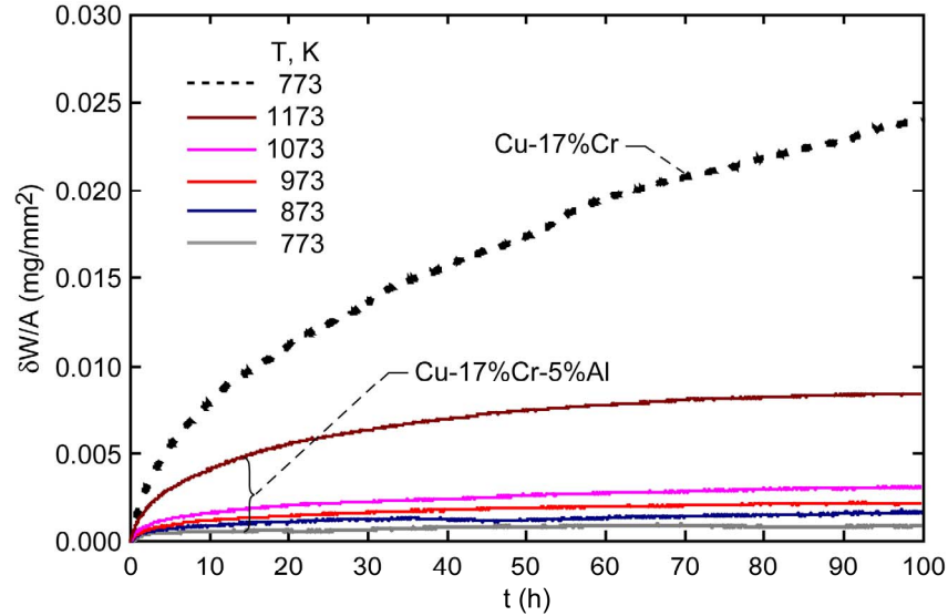
Figure 4.—Comparison of the specific weight change data for Cu-17%Cr determined at 773 K with those for Cu-17%Cr-5%Al determined between temperatures (T) 773 and 1173 K, demonstrating the superior oxidation behavior of the Al-containing alloy.
