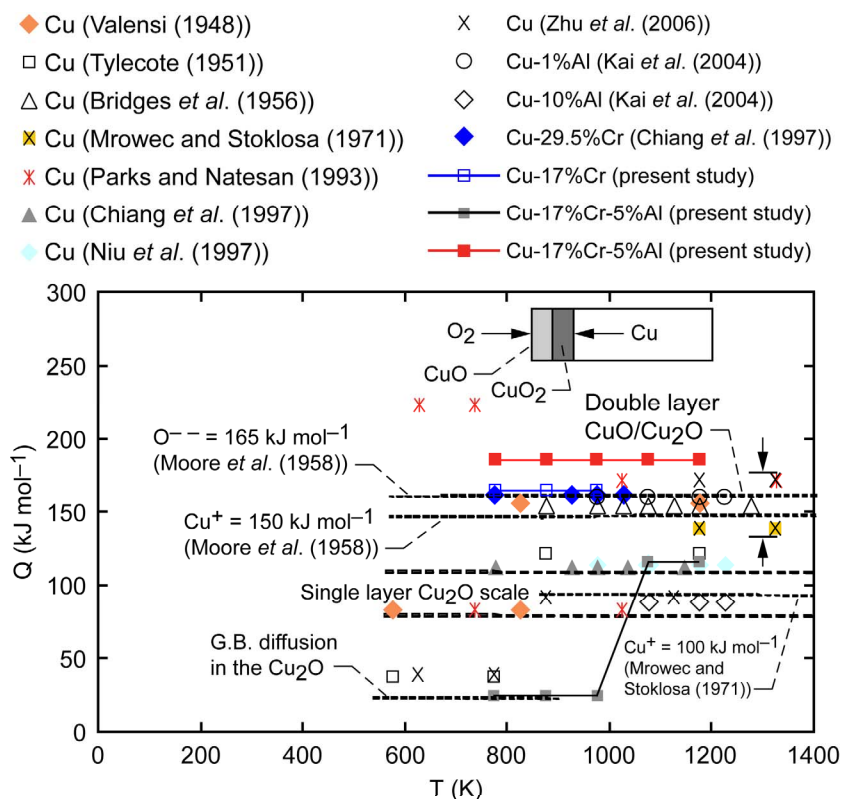
Figure 9.—Comparison of the activation energies for oxidation of pure Cu (refs. 6, 9, 10, 16, 19, 20, 21, and 22), Cu-Al (48), and Cu-29.5%Cr (21) with those for Cu-17%Cr and Cu-17%Cr-5%Al. The lower values of activation energies for oxidation of Cu-17%Cr-5%Al were determined using the parabolic relationship, whereas the higher values were determined from the quartic relationship.
