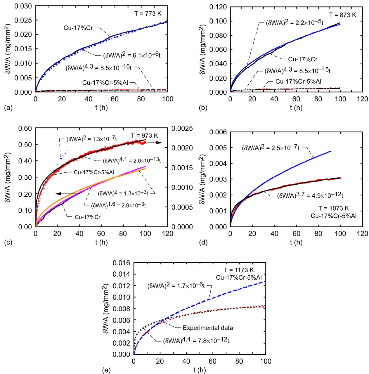
Figure 6.—Comparison of the regression equations with experimental data for Cu-17%Cr and Cu-17%Cr-5%Al at different temperatures (T). (a) 773 K. (b) 873 K. (c) 973 K. (d) 1073 K. (e) 1173 K.
