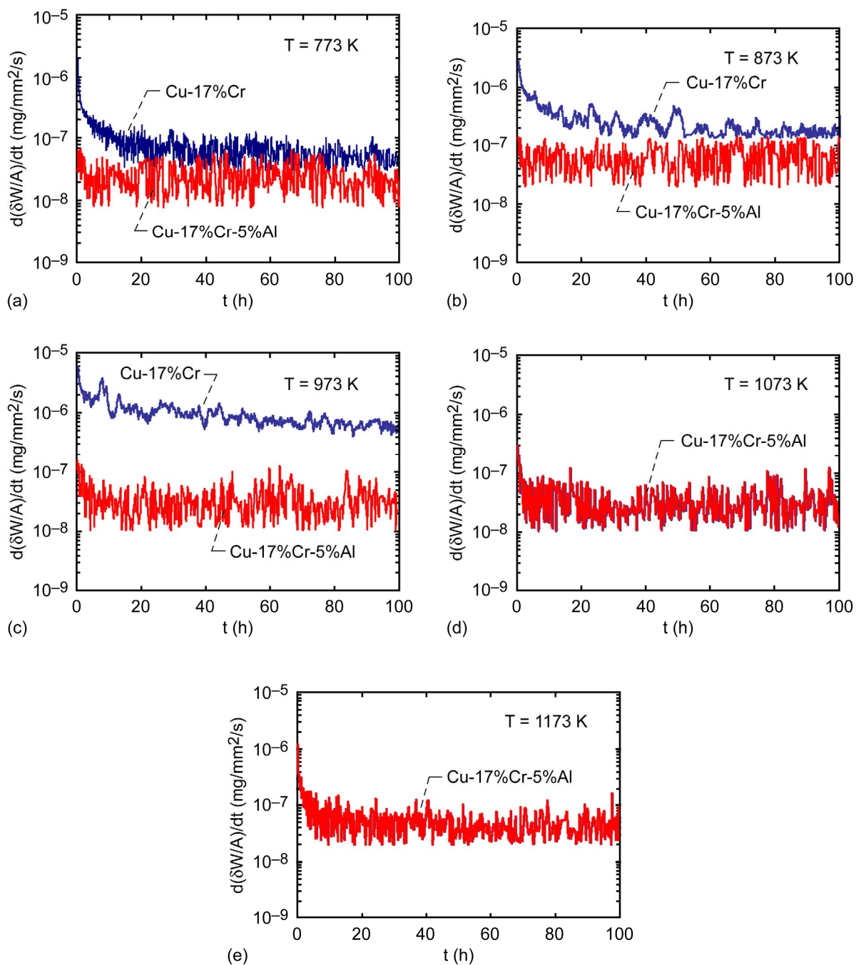
Figure 3.—Variation of the rate of the specific weight change with time for Cu-17%Cr and Cu-17%Cr-5%Al at different temperatures ( T ). (a) 773 K. (b) 873 K. (c) 973 K. (d) 1073 K. (e) 1173 K.
