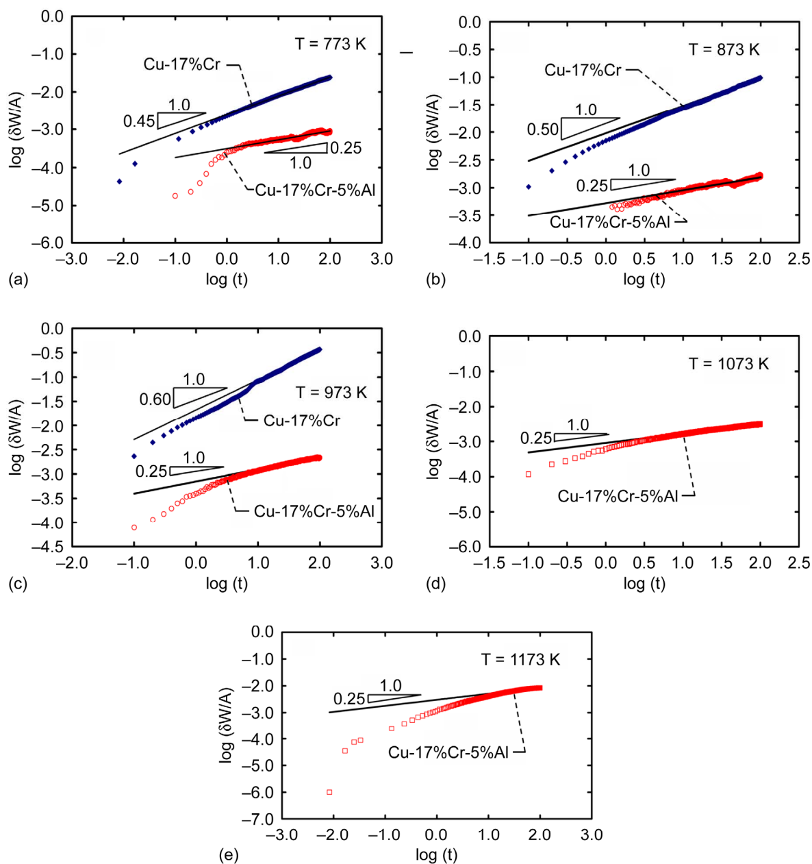
Figure 5.—Double logarithmic plots showing the variation of the specific weight change with time for Cu-17%Cr and Cu-17%Cr-5%Al at different temperatures (T). (a) 773 K. (b) 873 K. (c) 973 K. (d) 1073 K. (e) 1173 K.
