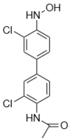
N-hydroxy-N'-acetyl-dichlorobenzidine
