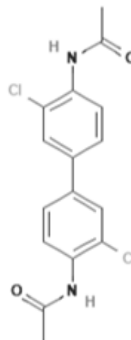
N,N'-diacetyl-3,3'-dichlorobenzidine
