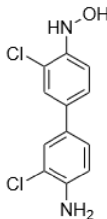
N-hydroxy-Dichlorobenzidine
