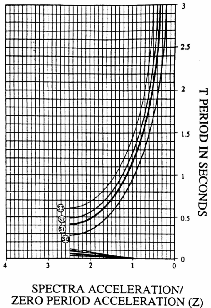
FIGURE NO. 3 NORMALIZED RESPONSE SPECTRA 5% DAMPING
