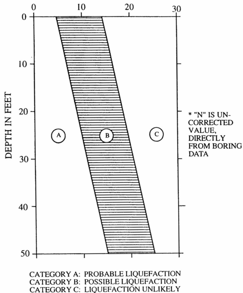
FIGURE NO. 4 "N" IN BLOWS PER FOOT*
