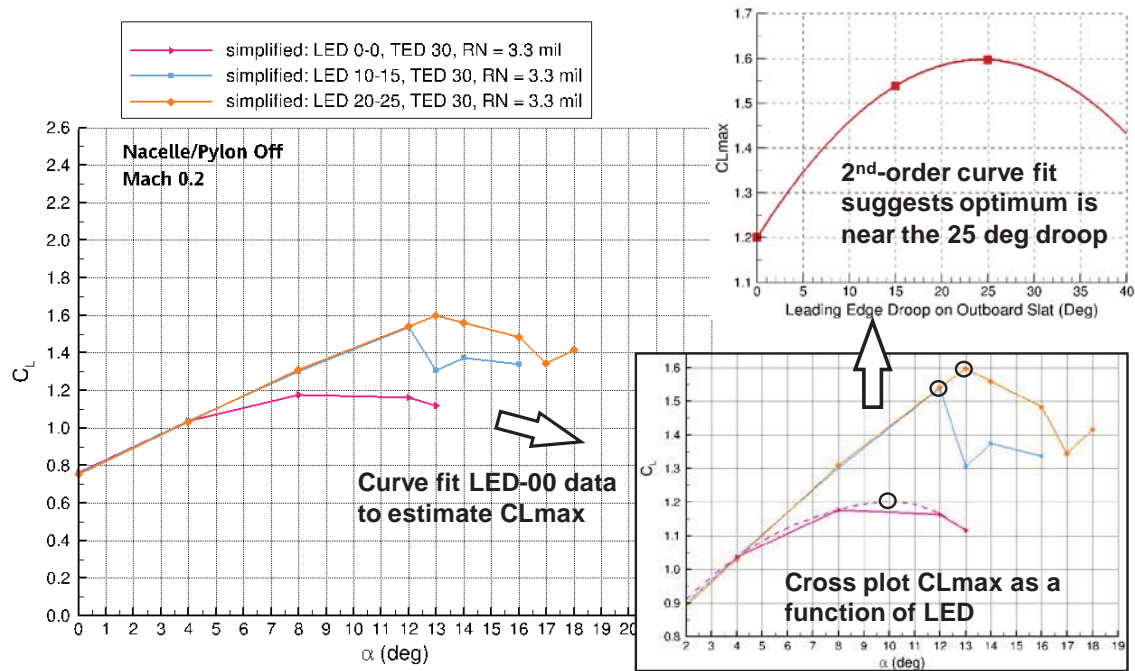
Figure 17 Lift curve comparisons for simplified high-lift CRM wing/body configuration indicate 25-degree leading-edge droop to be near optimum setting.
