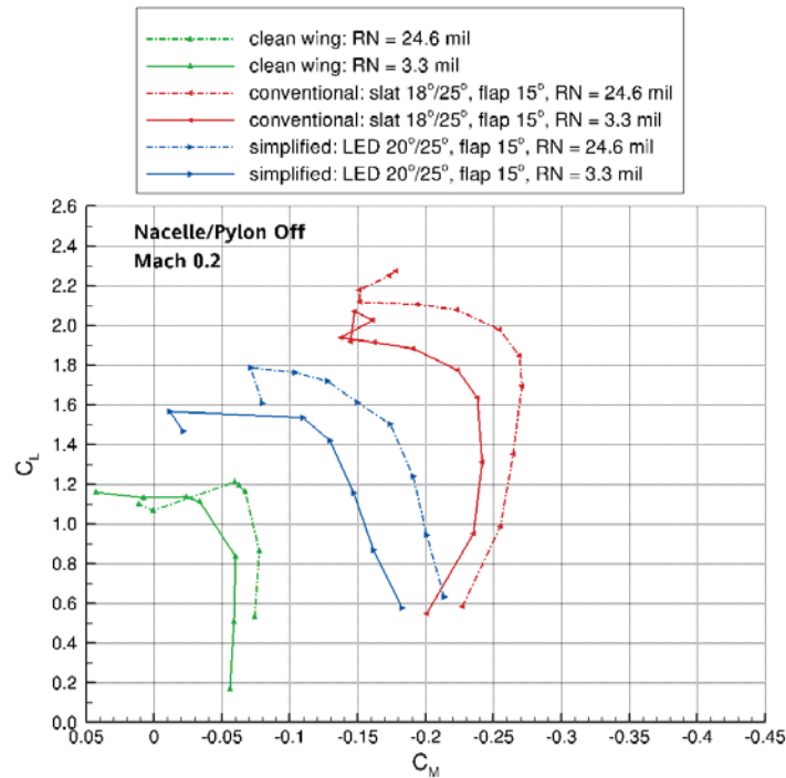
Figure 20 Pitching-moment comparisons – clean vs. takeoff high-lift CRM configurations (conventional & simplified).
