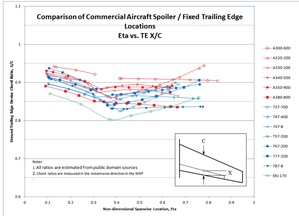
Figure 7 CRM spoiler-to-wing trailing edge chord ratio is in Family with control surface layouts on current fleet commercial transport aircraft.
