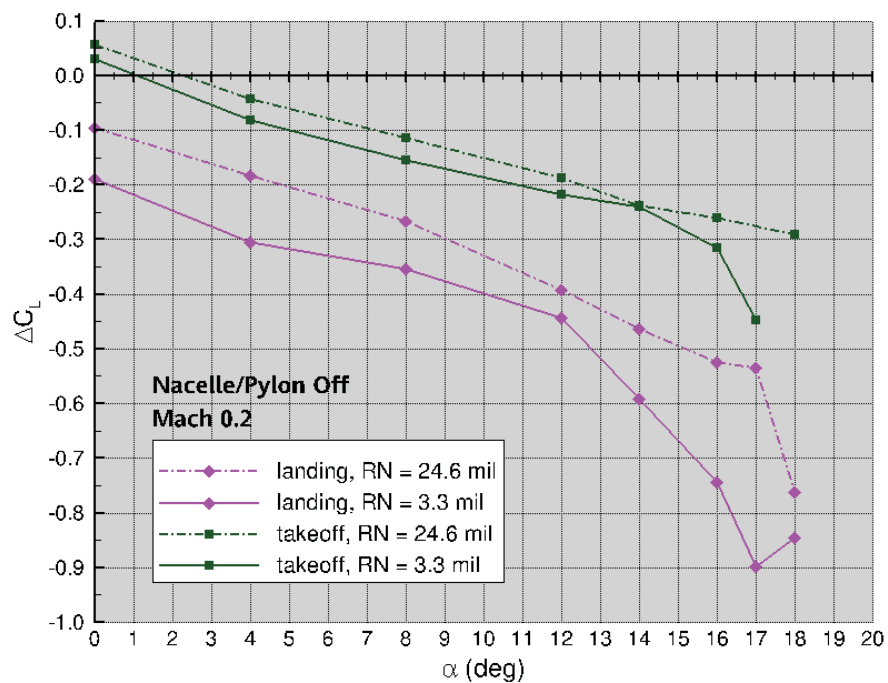
Figure 18 Incremental-lift comparisons between conventional and simplified high-lift CRM configurations.
