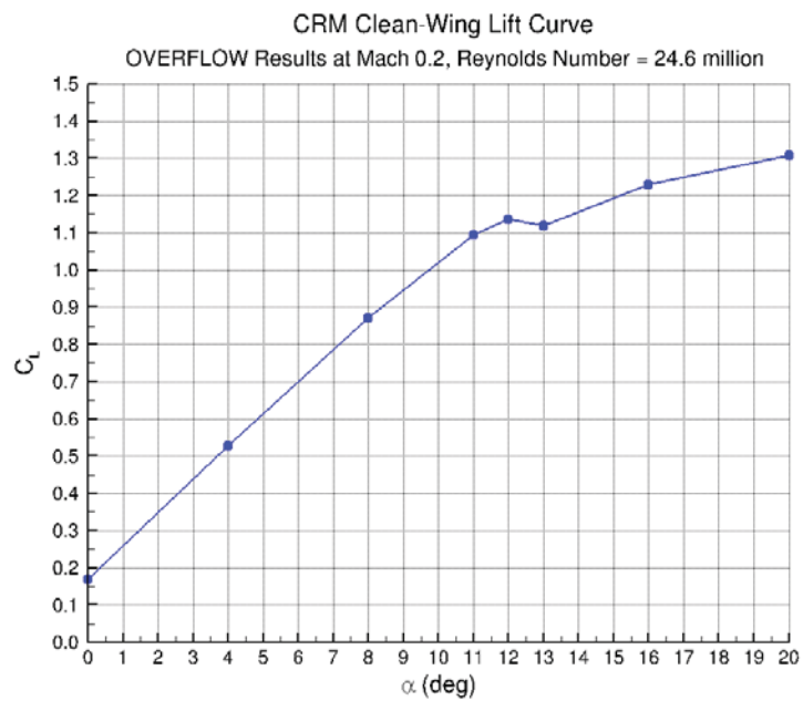
Figure 10 Variation of lift with angle of attack for a clean (i.e., all high-lift devices retracted) high-lift CRM wing/body/nacelle/pylon configuration..
