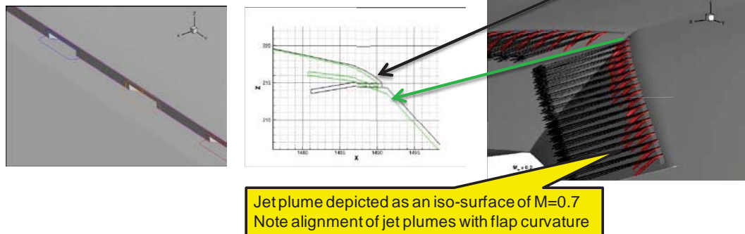
Figure 26 Convergent-divergent ducts are used to model fluidic oscillators for discrete-blowing AFC simulation.
