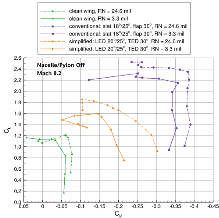
Figure 19 Pitching-moment comparisons – clean vs. landing-approach high-lift CRM configurations (conventional & simplified).
