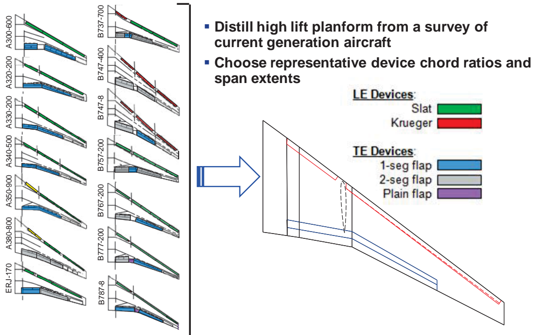
Figure 4 High-lift systems on current fleet aircraft trend toward combining slats with single-element slotted flaps.
