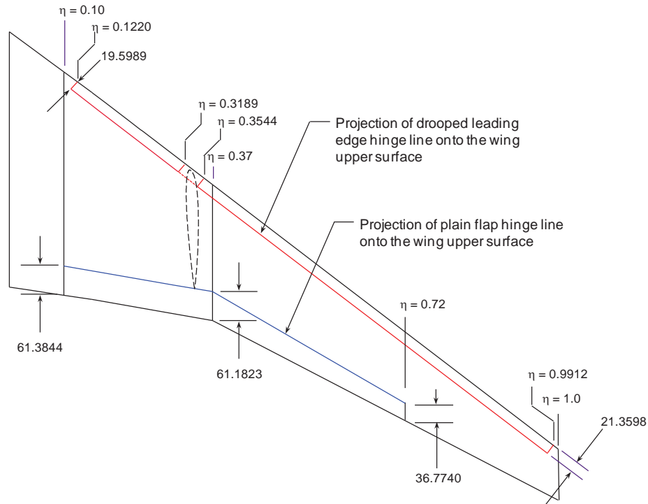
Figure 9 Conventional and simplified high lift system planform definitions are matched to promote meaning high-lift aerodynamics comparisons.
