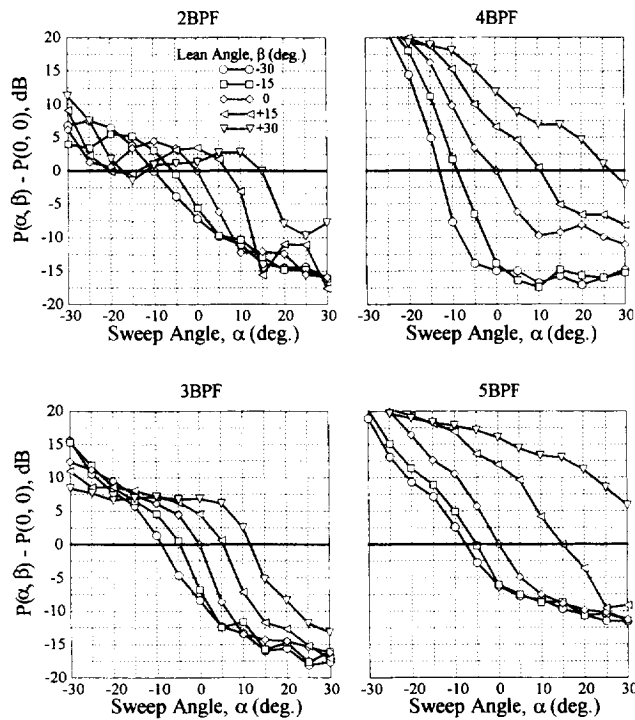
Figure 6. Influence of sweep and lean on the in-duct tone power. Cutback condition (upstream noise).
