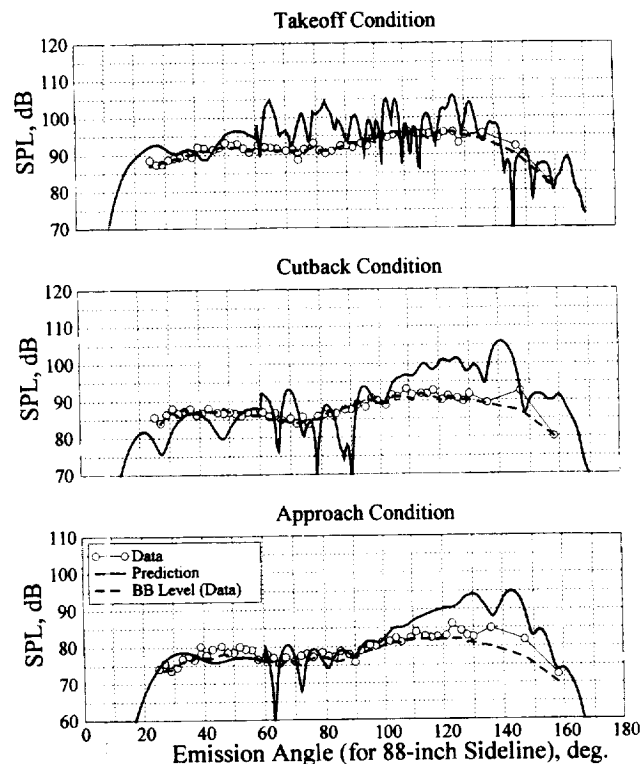
Figure 17. Comparison of measured and predicted 2BPF tone farfield directivities for the swept and leaned stator. Measured broadband noise level around 2BPF tone is also shown.
