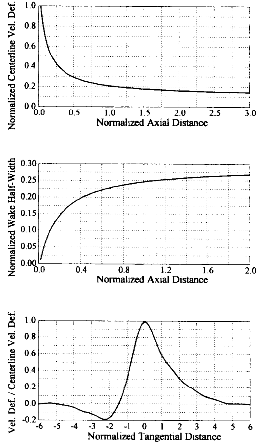
Figure 3. Rotor wake characteristics used in this study.
