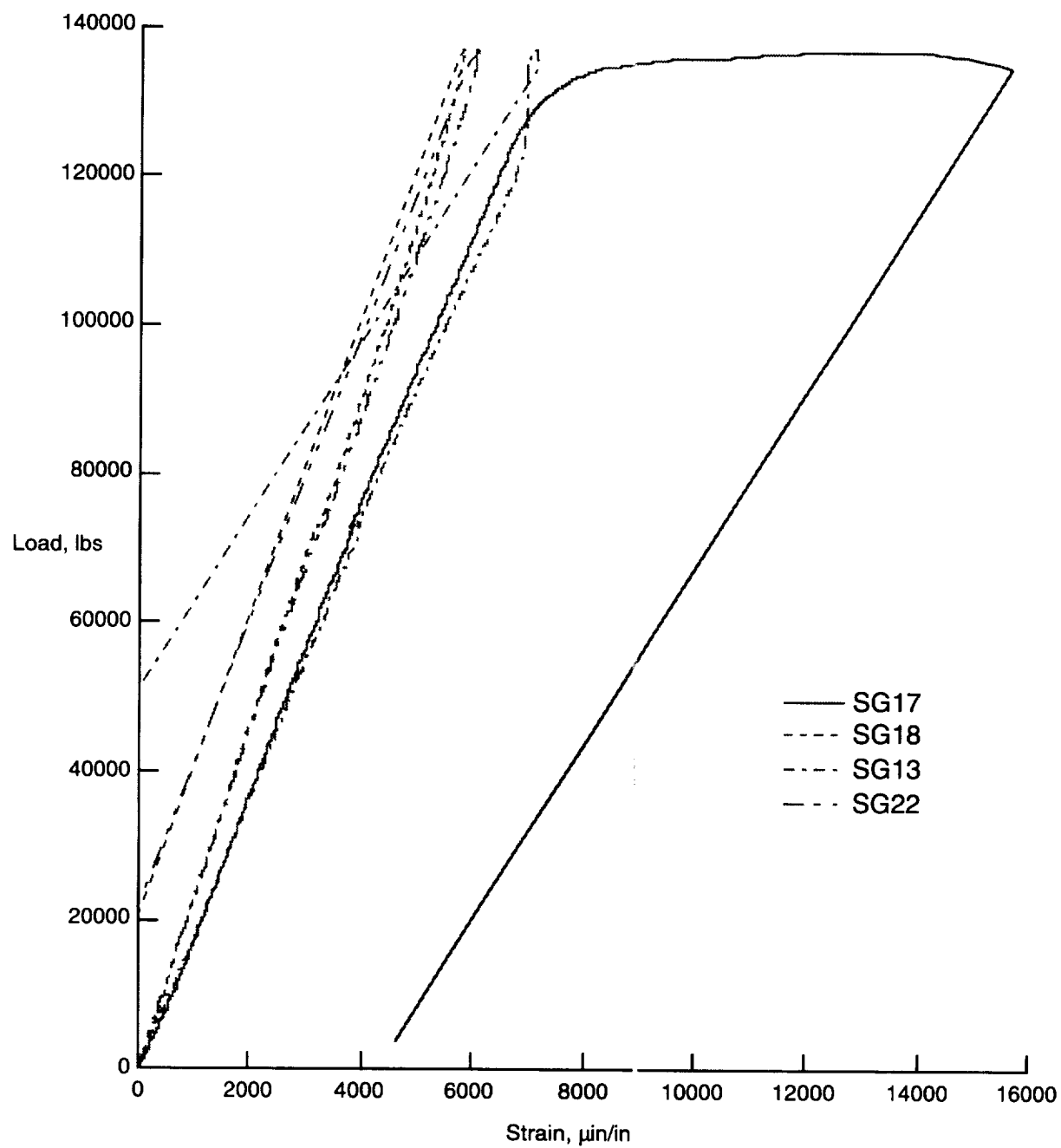
Figure 19. Strains measured at the center of the splice plate for the PMC to PMC joint specimen tested at room temperature.
