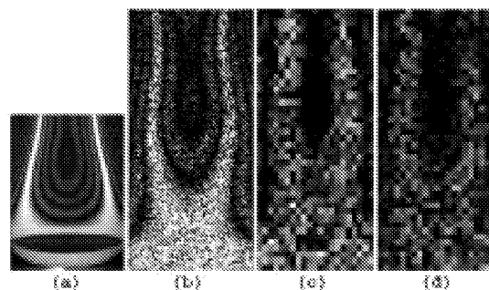
Fig. 8. First chord-wise mode: (a) from a silver halide hologram of a vibrating blade, (b) from electronic holograms of a vibrating cantilever, (c) from a finite-element-resolution model of a cantilever plate, (d) from electronic holograms at finite-element resolution.
