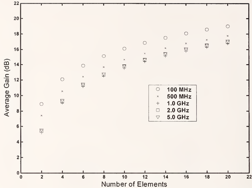
Figure 28. Average gain using 1000 trials and 24 random observation positions over 10 m perimeter random radiation elements in a volume 25 m \times 25 m \times 1.4 m; z positions range over the interval [0.1 m, 1.5 m].
