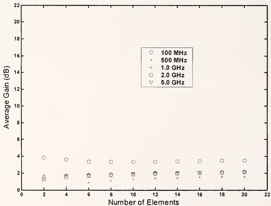
Figure 14. Average gain using uniformly distributed random phase with unity magnitude currents for 1000 trials and 24 random positions over 16 \text{ m} \times 16 \text{ m} square area in the z = 1.3 \text{ m} plane.
