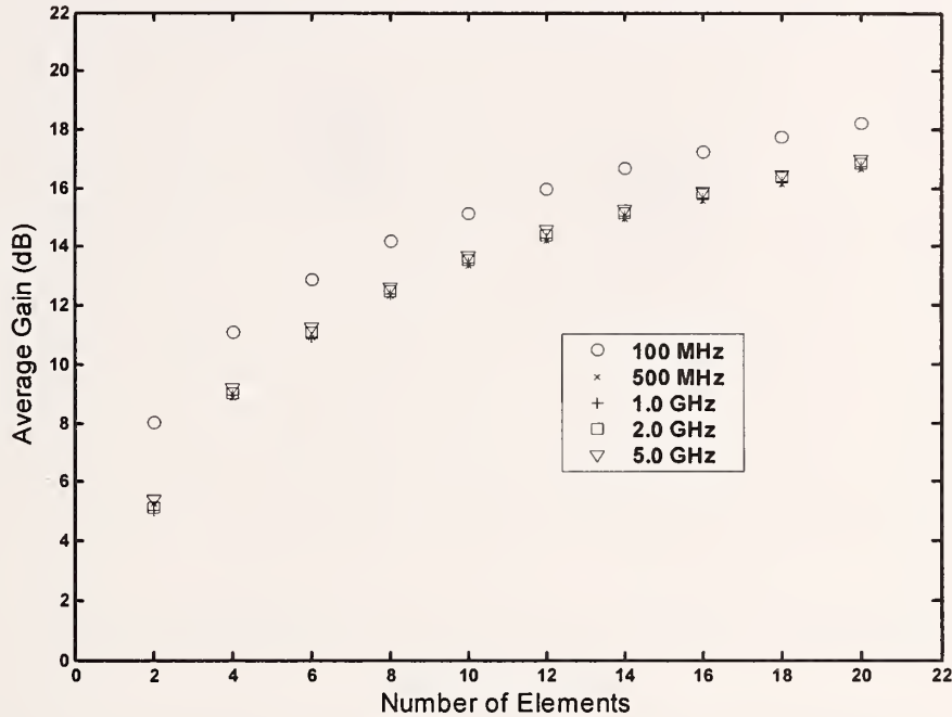
Figure 22. Average gain using 1000 trials and 24 random observation positions over 16 \text{ m} \times 16 \text{ m} square area; random radiation elements in a volume 25 \text{ m} \times 25 \text{ m} \times 1.4 \text{ m} ; z positions range over the interval [0.1 \text{ m}, 1.5 \text{ m}] .
