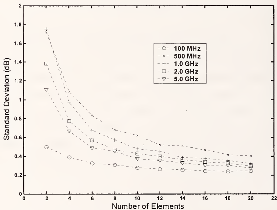
Figure 24. Standard deviation of average gain results shown in figure 21.
