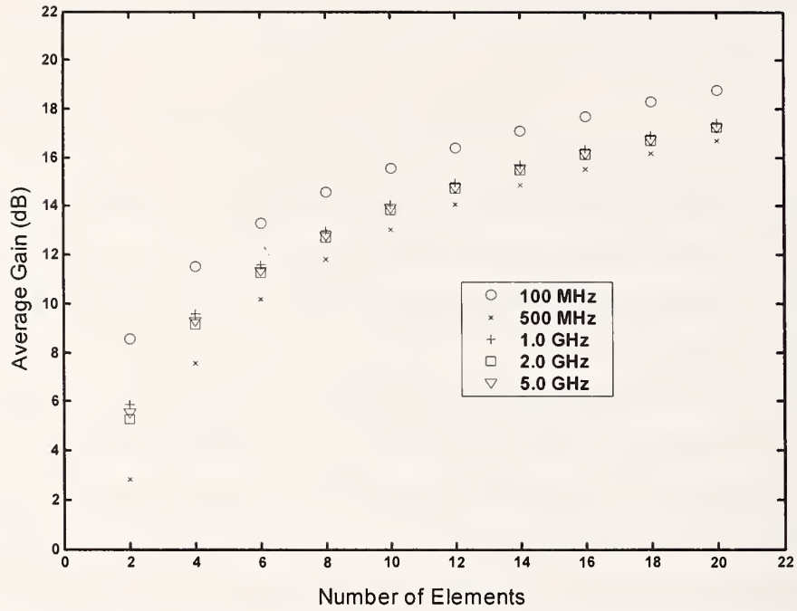
Figure 6. Average gain using 1000 trials and 24 random observation positions over 16 m \times 16 m square area.
