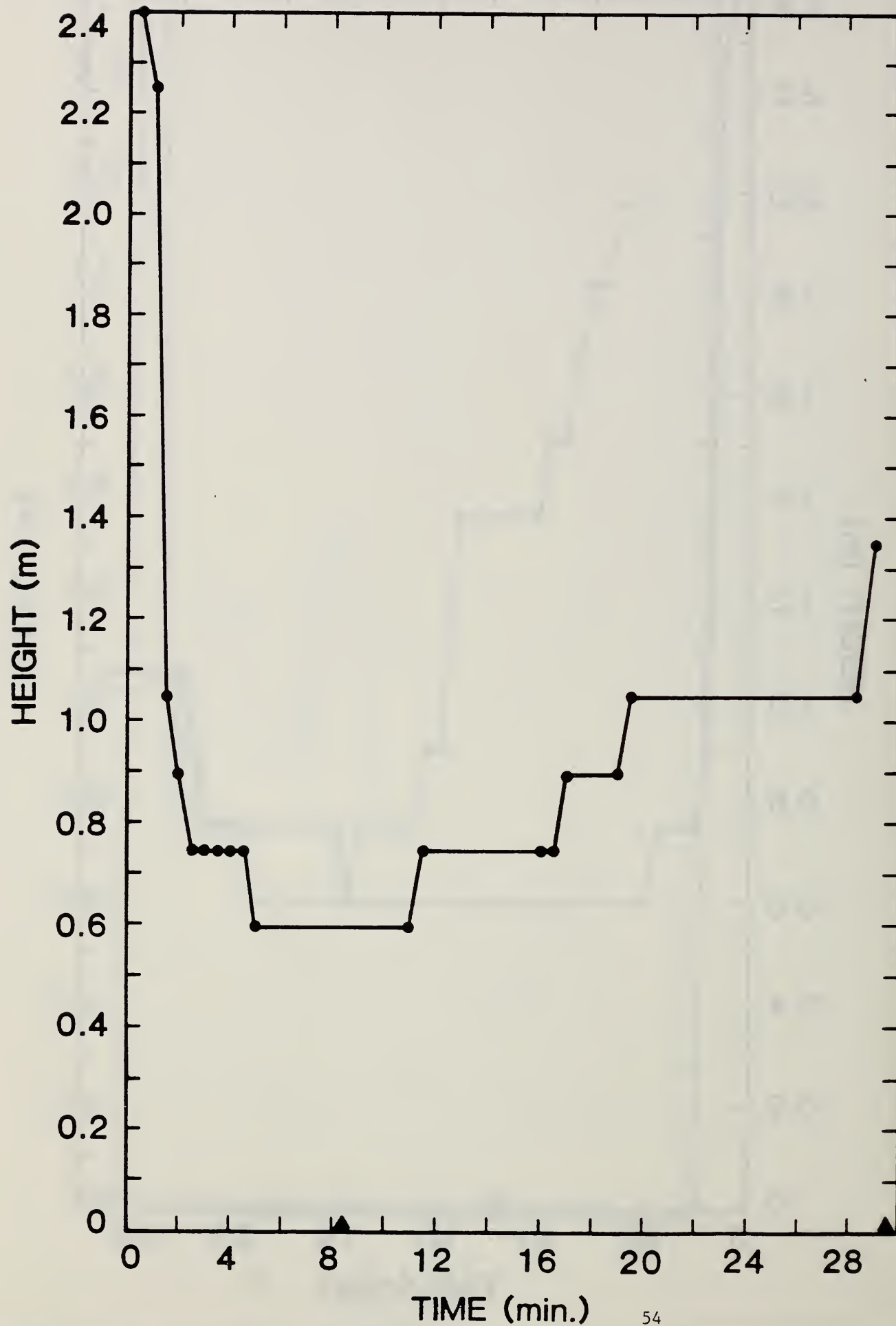
Figure 34. Depth of Lower Layer Test Number 5
