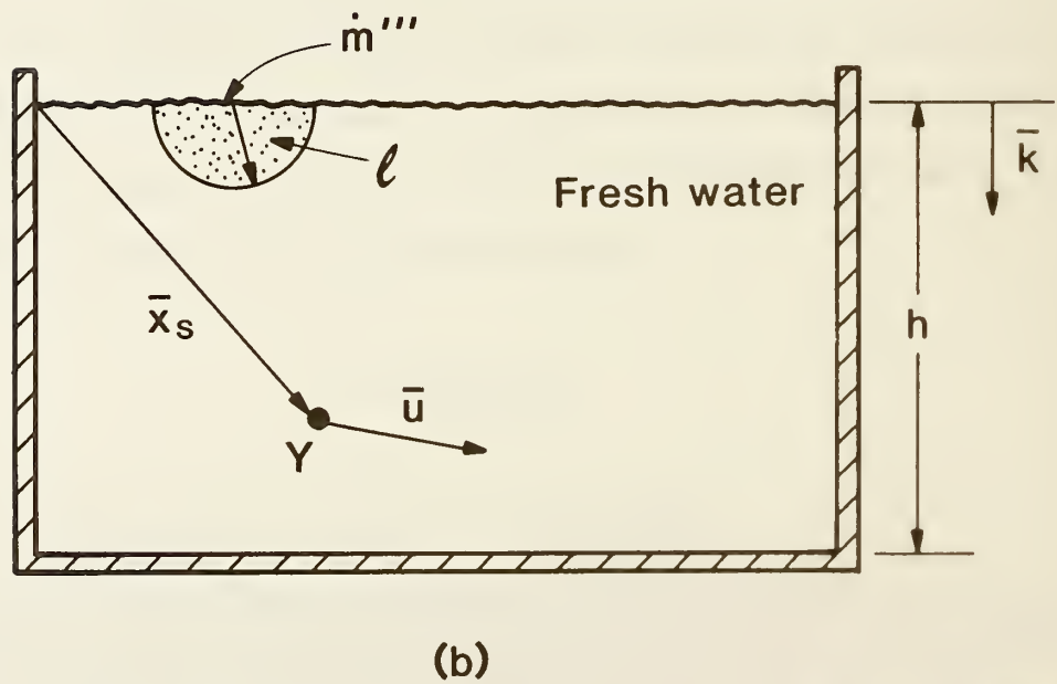
Fig. 1. Enclosures; (a) full-scale with heat source, (b) reduced-scale with salt water source.
