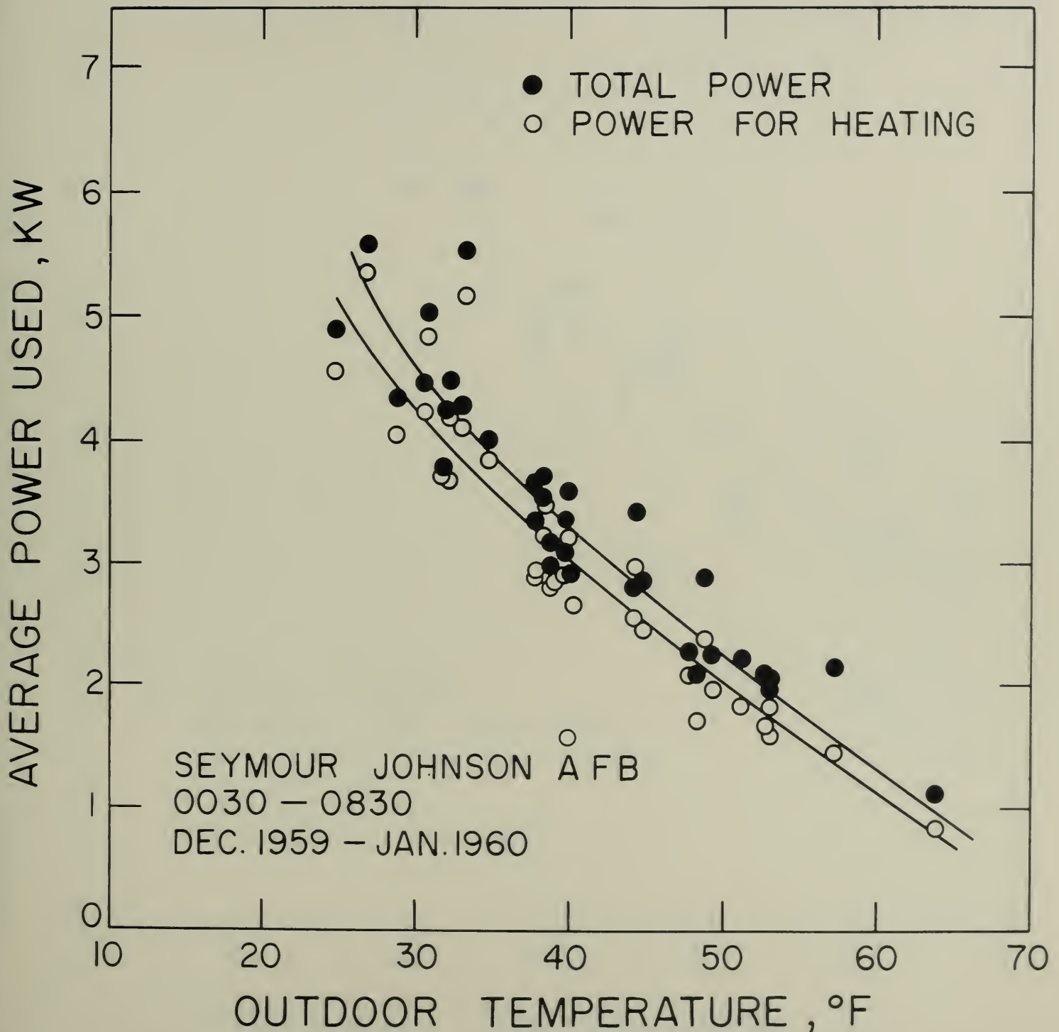
Fig. 45. Average Power Used for Heating and for All Purposes During the Hours 0030 to 0830 in the Five Sample Houses at Seymour Johnson AFB, for a Range of Outdoor Temperature
