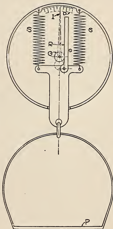
FIG. 5.—Diagram of the spring balance
