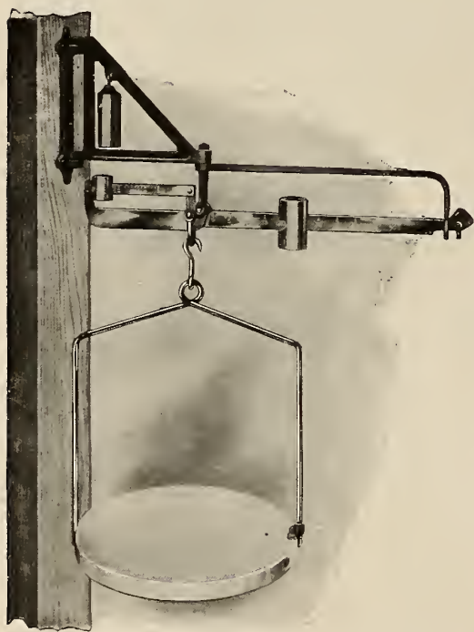
FIG. 6.—Folding household scale of the steelyard type
