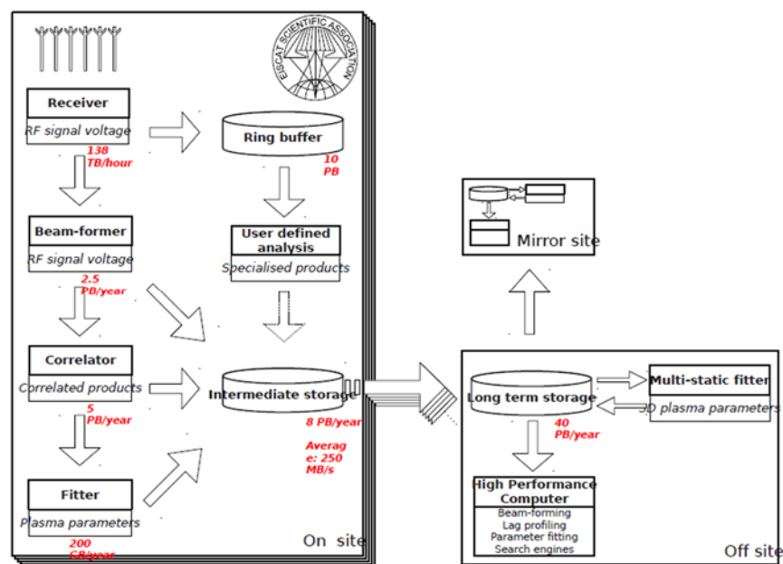
Figure 8: EISCAT 3D Incoherent Scatter Radar System – System Architecture
