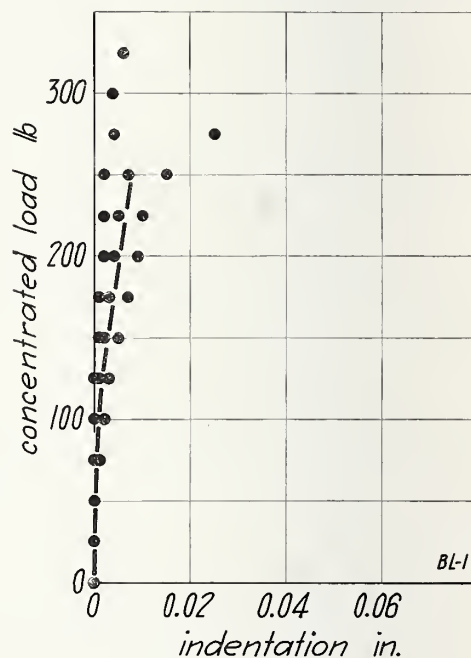
FIGURE 65.—Concentrated load on wall BL, load applied to inside face.
