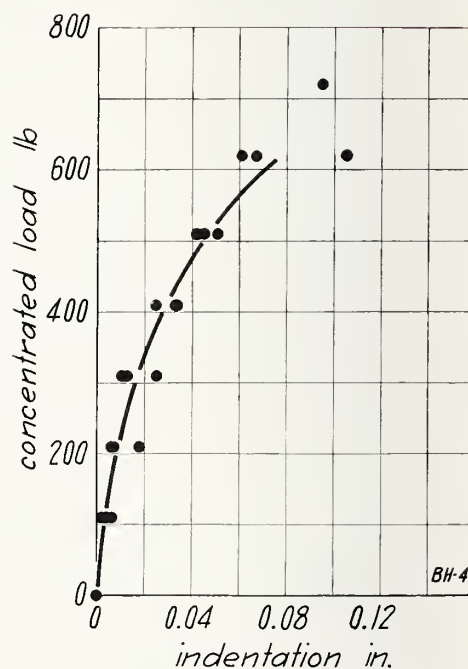
FIGURE 24.—Concentrated load on wall BH, load applied to outside face.
