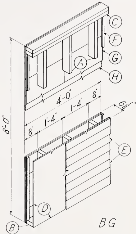
FIGURE 5.—Four-foot wall specimen BG.
