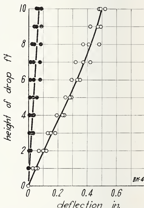
FIGURE 58.—Impact load on wall BK, load applied to outside face.
