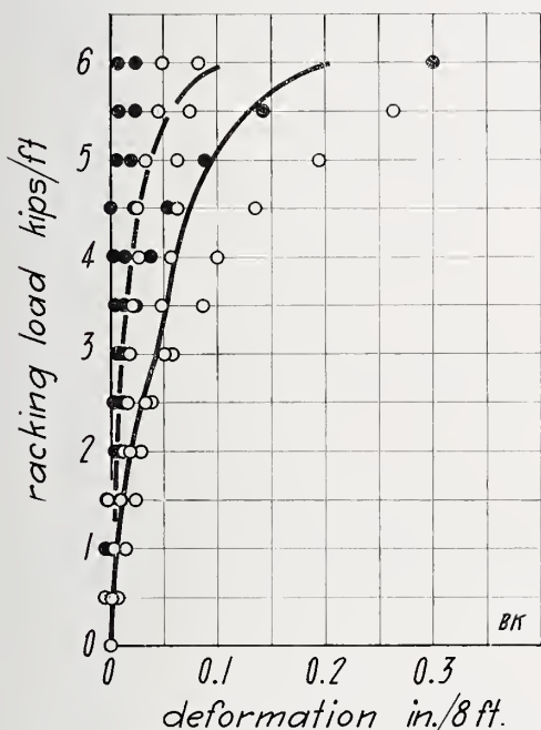
FIGURE 59.—Racking load on wall BK .
