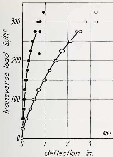
FIGURE 53.—Transverse load on wall BK, load applied to inside face.
