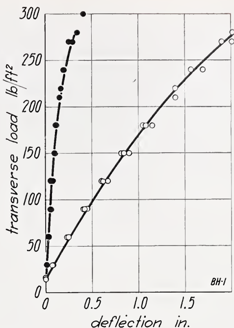
FIGURE 20.—Transverse load on wall BH-I , load applied to inside face.
