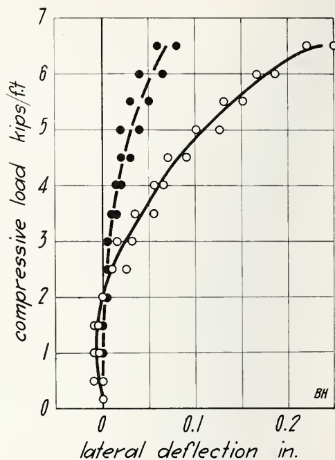
FIGURE 19.—Compressive load on wall BH.
