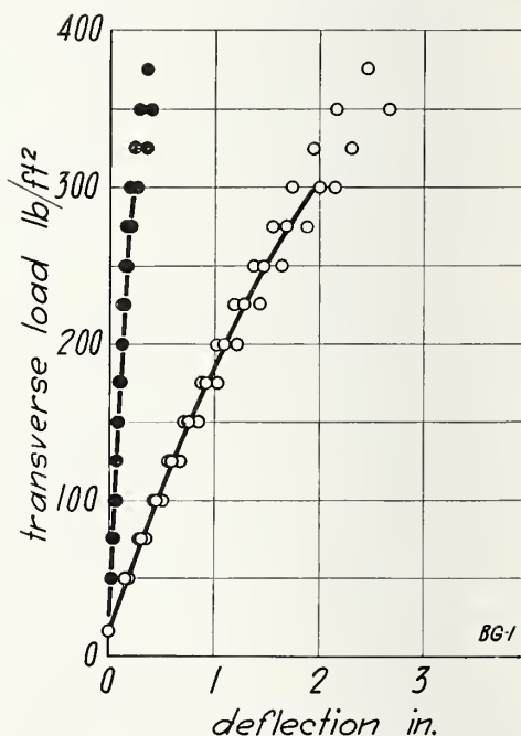
FIGURE 9. Transverse load on wall BG, load applied to inside face.
