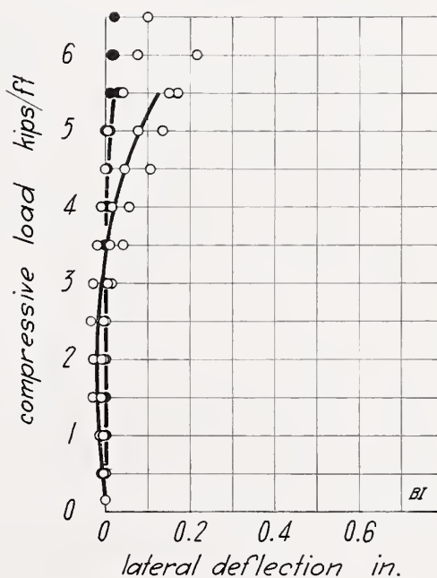
FIGURE 29.—Compressive load on wall BI .
