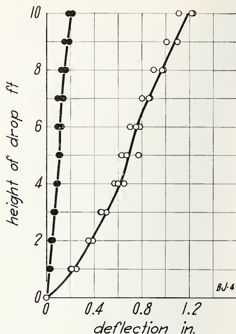
FIGURE 47.—Impact load on wall BJ , load applied to outside face.
