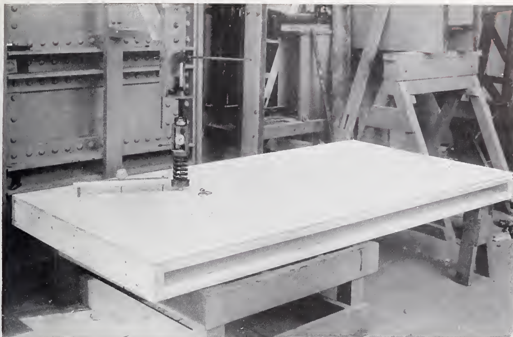
FIGURE 73.—Partition specimen BM-P2 under concentrated load.
