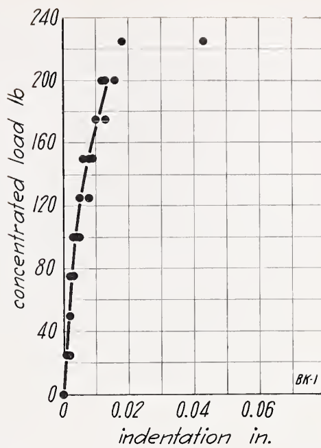
FIGURE 55.—Concentrated load on wall BK, load applied to inside face.
