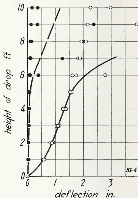
FIGURE 36.—Impact load on wall BI , load applied to outside face.
