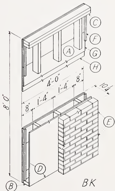
FIGURE 49.—Four-foot wall specimen BK .
