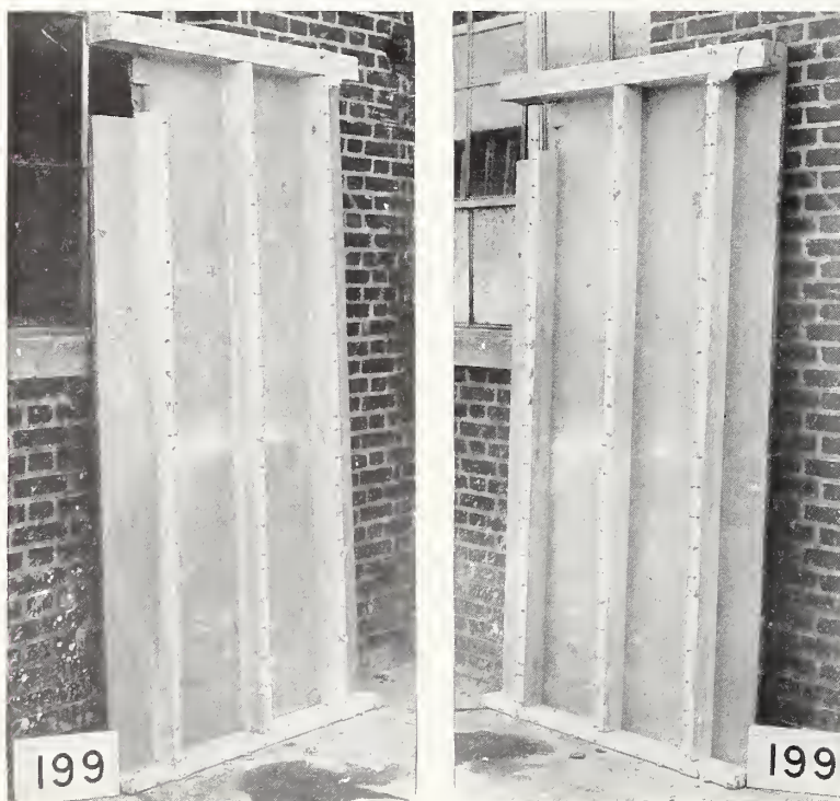
FIGURE 1.—Frame of wall specimen BK-14.
