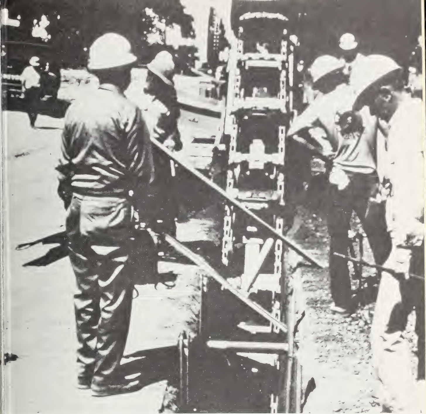
Trenching machine used in trench braced by hydraulic shores
